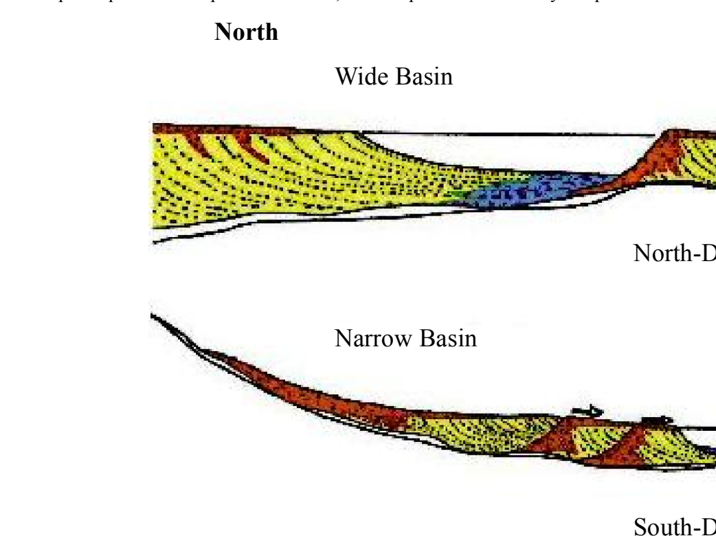
Figure 2: Scenario for morphosequence development in ice-dammed (Top) and sediment-dammed basins (Bottom). The mechanism of impoundment and the chronological and topographic positions of the deposits are related to the orientation of the basins relative to the direction of ice retreat. These relationships are reflected in the organization and color coding of the List of Map Units (after Stone and others, 2005).
