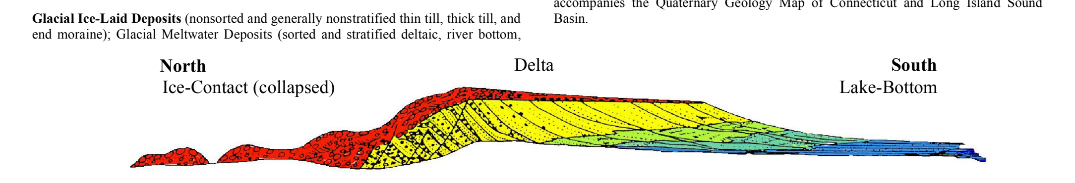
Figure 1: A morphosequence is a body of meltwater deposits composed of a continuum of land forms, grading from ice-contact forms (eskers, kames) to non-ice-contact forms (flat valley floor, delta plains), that were deposited simultaneously as and beyond the margin of a glacier, graded to a specific base level. Grain-size decreases from coarse gravel at ice-contact, through sand and gravel and silt beneath delta plains and forest slopes to silt and clay in lake-bottom deposits (after Stone and others, 2005).
