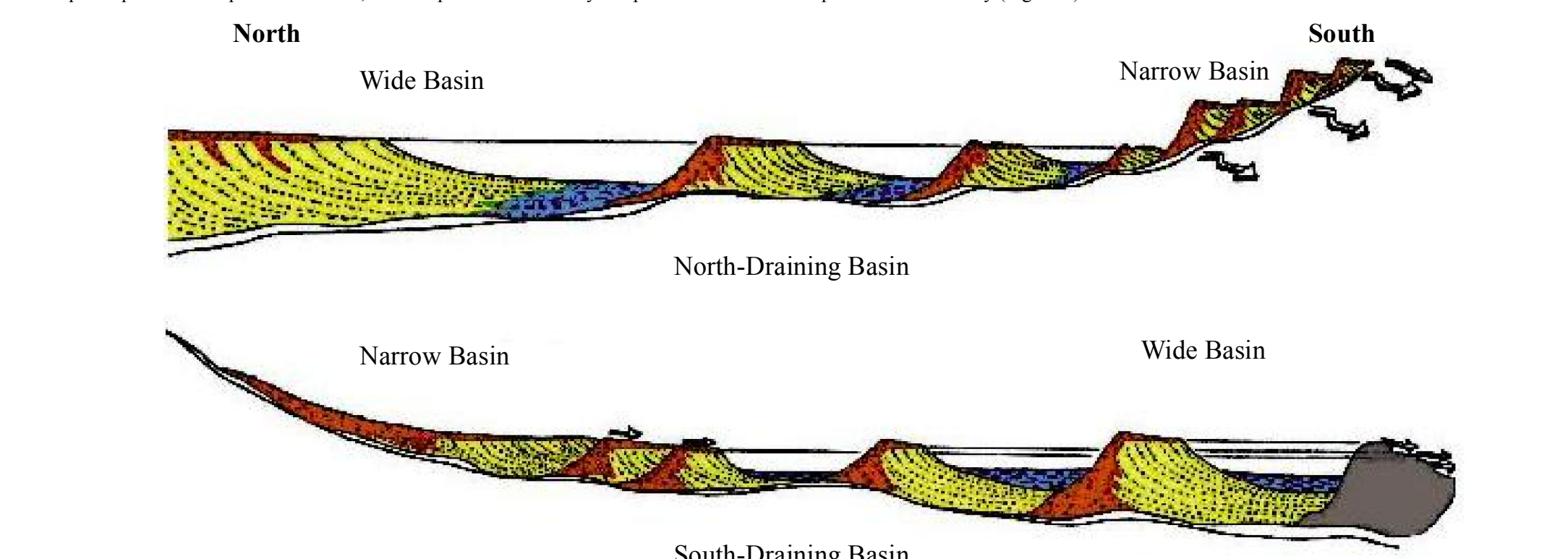
Figure 2: Scenario for morphosequence development in ice-dammed (Top) and sediment-dammed basins (Bottom). The mechanism of impoundment and the chronological and topographic relationships of the deposits are related to the orientation of the basin relative to the direction of ice retreat. These relationships are reflected in the organization and color coding of the List of Map Units (after Stone and others, 2005).
