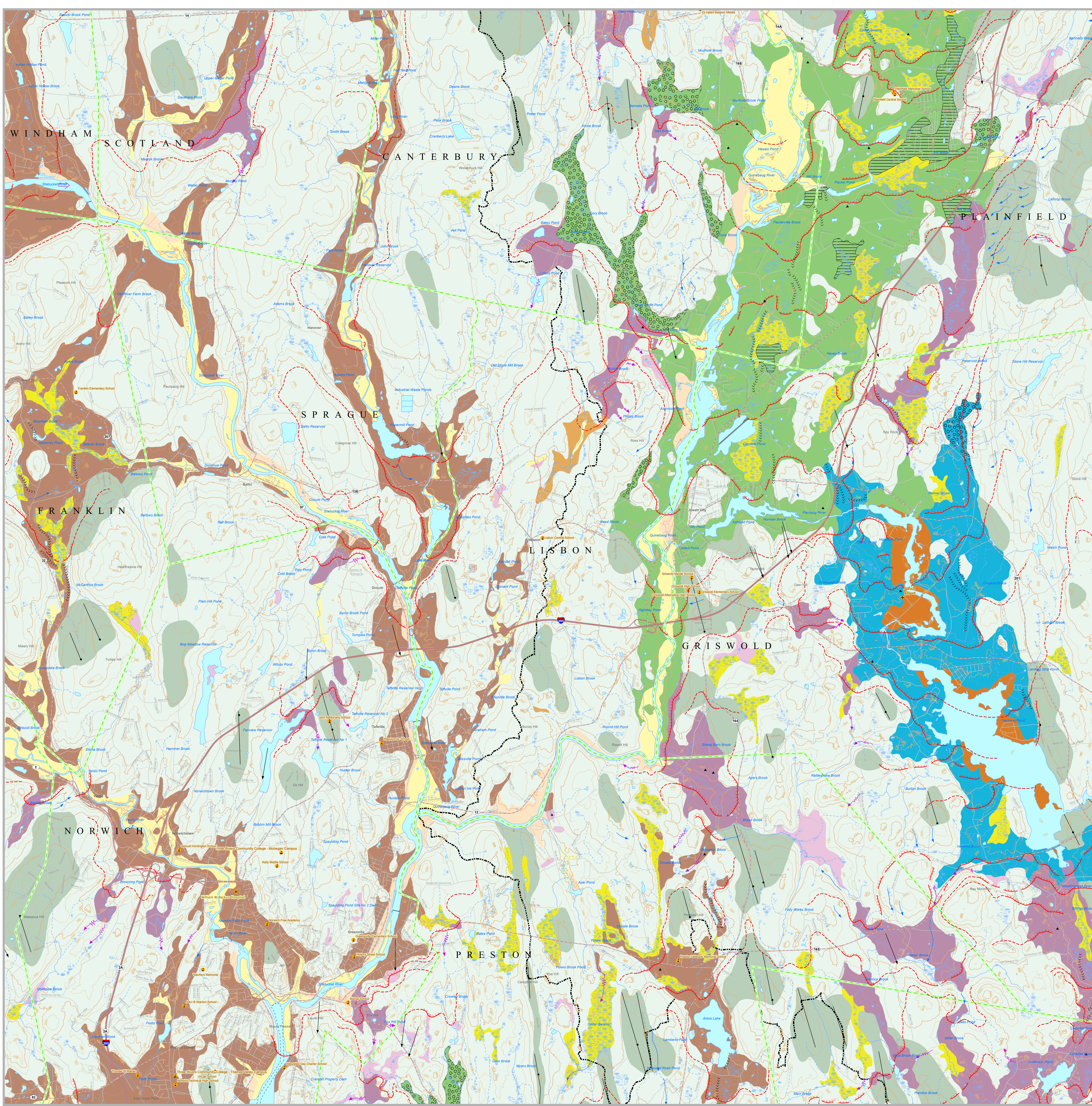
Figure 1: A morphosequence is a body of meltwater deposits composed of a continuum of land forms, grading from ice-contact forms (eskers, kames) to non-ice-contact forms (flat valley floor, delta plains), that were deposited simultaneously as and beyond the margin of a glacier, graded to a specific base level. Grain-size decreases from coarse gravel at ice-contact, through sand and gravel and silt beneath delta plains and forest slopes to silt and clay in lake-bottom deposits (after Stone and others, 2005).
