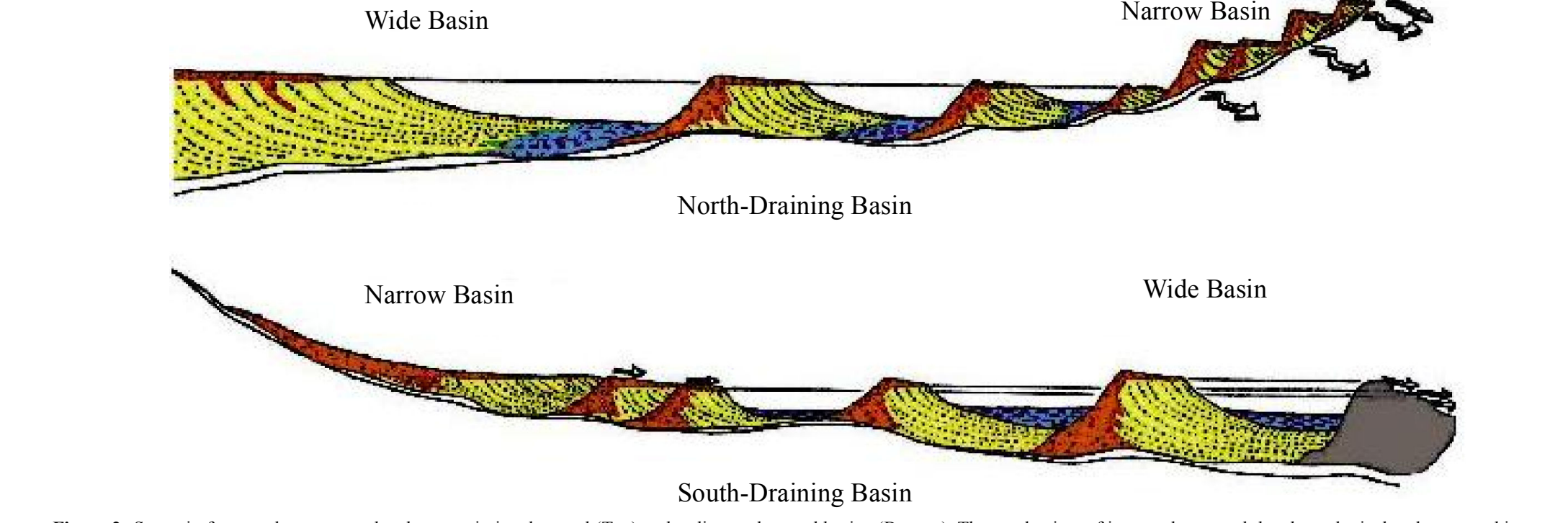
Figure 2: Scenario for morphosequence development in ice-dammed (Top) and sediment-dammed basins (Bottom). The mechanism of impoundment and the chronological and topographic positions of the deposits are related to the orientation of the basin relative to the direction of ice retreat. These relationships are reflected in the organization and color coding of the List of Map Units (after Stone and others, 2005).
