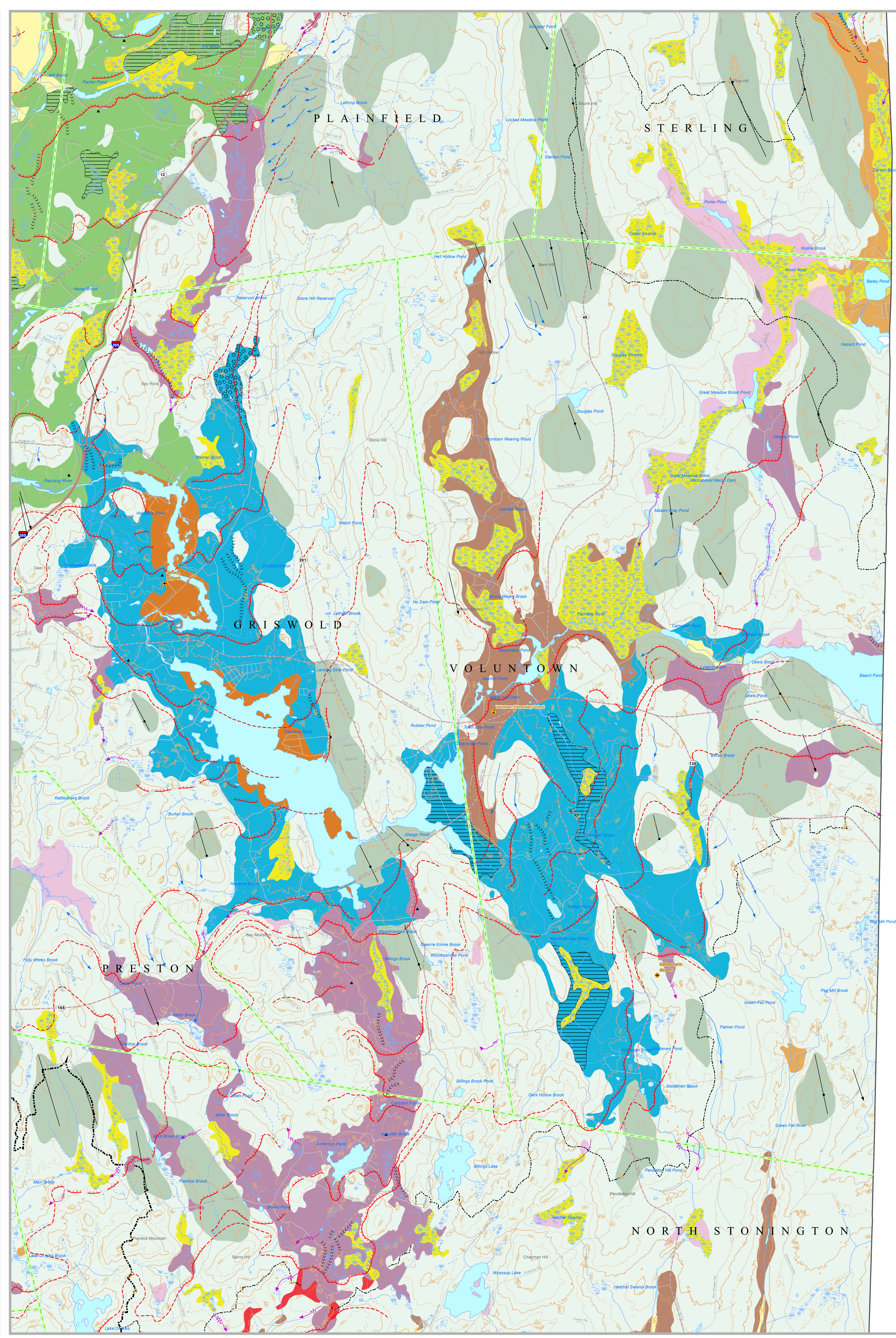
Figure 1. A morphosequence is a body of meltwater deposits composed of a continuum of land forms, grading from ice-contact forms (eskers, kames) to non-ice-contact forms (flat valley terrace, delta plains), that were deposited simultaneously at and beyond the margin of a glacier, graded to a specific base level. Grain-size decreases from coarse gravel at ice-contact, through sand and silt beneath delta plains and forest slopes to silt and clay in lake-bottom deposits (after Stone and others, 2005).
